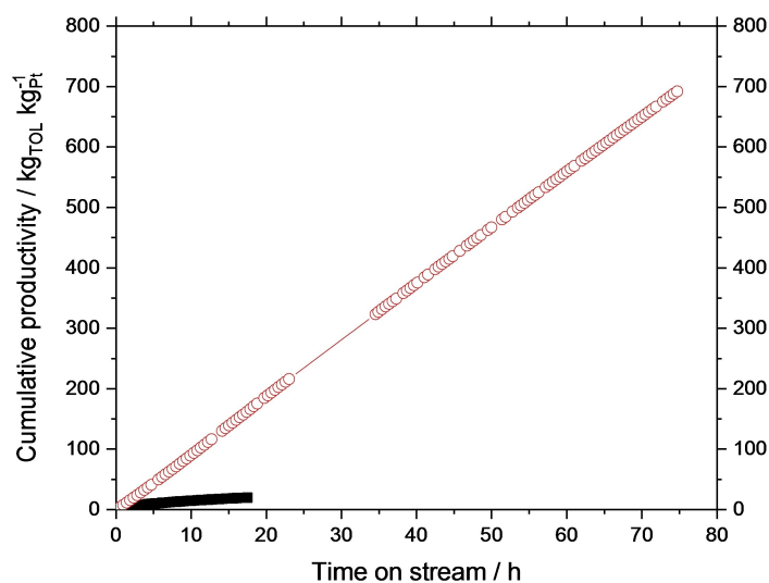
Figure 2. Dehydrogenation of methylcyclohexane (MCH) to toluene (TOL). Comparison between the cumulative productivity for toluene formation with \text{Pt}/\text{SiO}_2 (black) and \text{Ga}_{52}\text{Pt}/\text{SiO}_2 SCALMS (red) as catalysts. Reaction conditions: 4.2 mL catalyst bed volume, T = 450^\circ\text{C} , p_{\text{total}} = 1 \text{ bar} , \text{H}_2:\text{MCH}:\text{He} = 5:1:4 \text{ mol mol}^{-1} , gas hourly space velocity (GHSV) = 1730 \text{ h}^{-1} (under reaction conditions).
